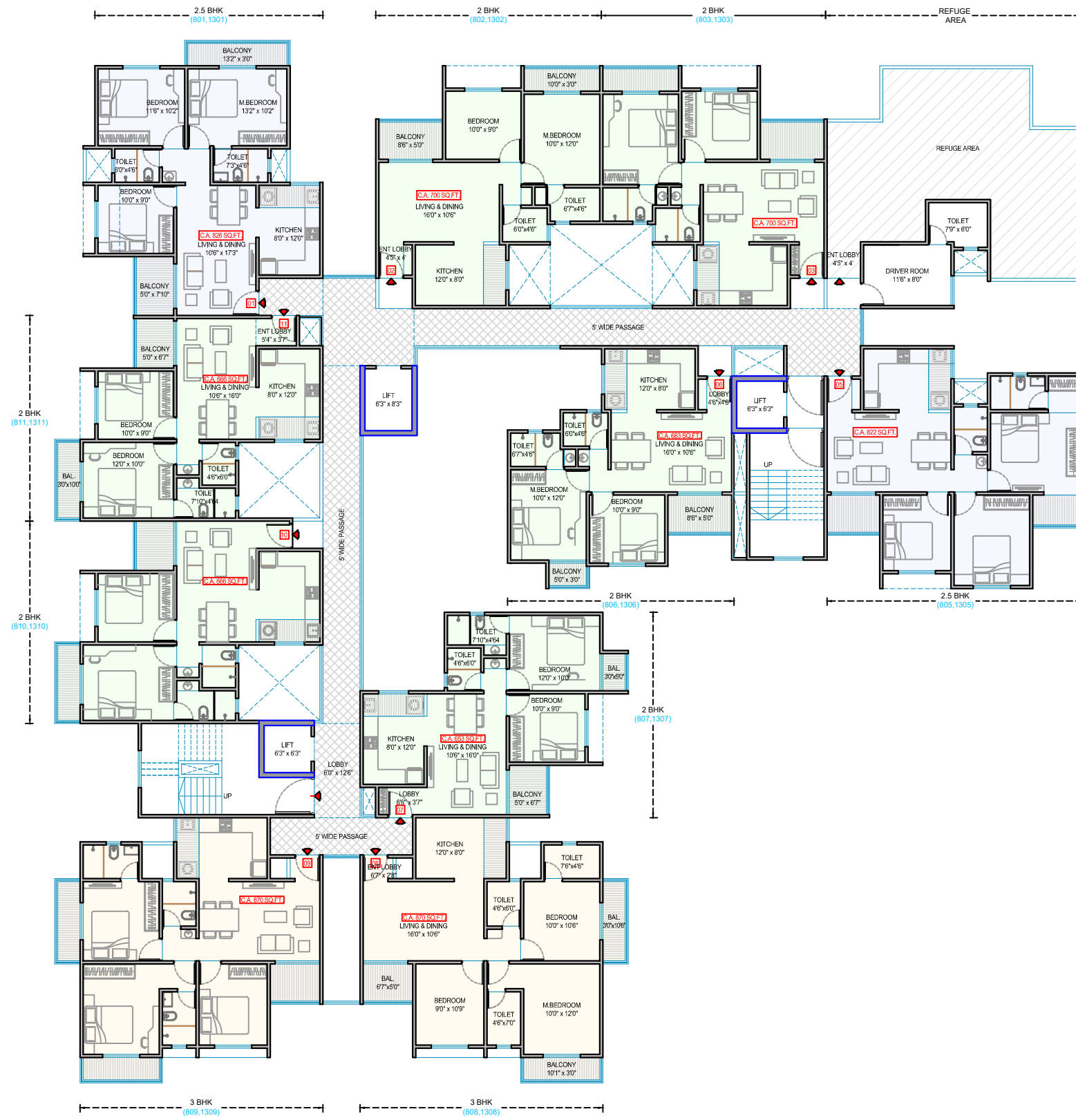
REFUGE FLOOR LAYOUT PLAN (TYPICAL 8TH & 13TH)
